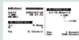
Typical roughness print out of surface after electropolishing
